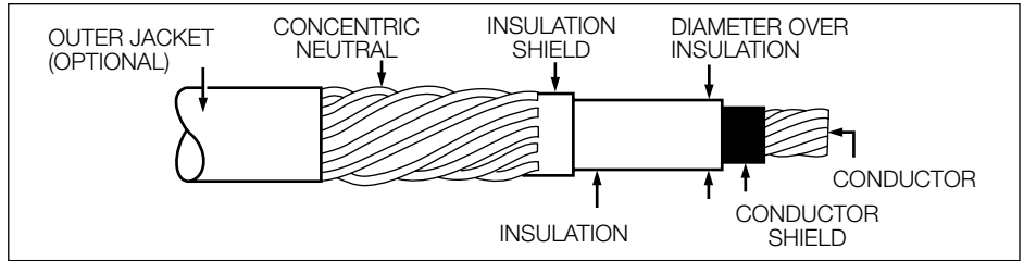
Figure 7. Cable cutaway showing conductor and insulation layers.
